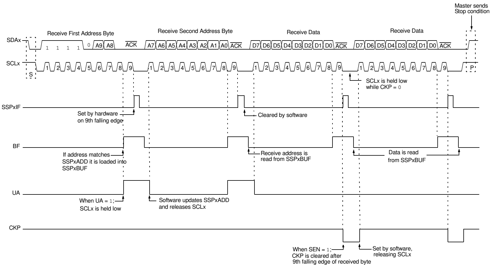
FIGURE 15-20: I 2 C SLAVE, 10-BIT ADDRESS, RECEPTION (SEN = 1, AHEN = 0, DHEN = 0)
