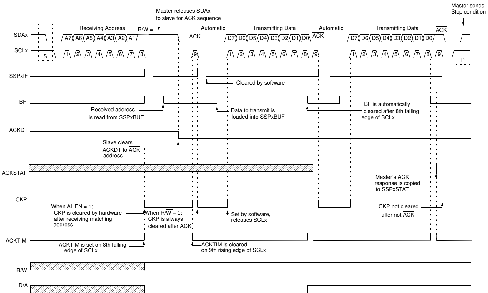
FIGURE 15-19: I 2 C SLAVE, 7-BIT ADDRESS, TRANSMISSION (AHEN = 1)
