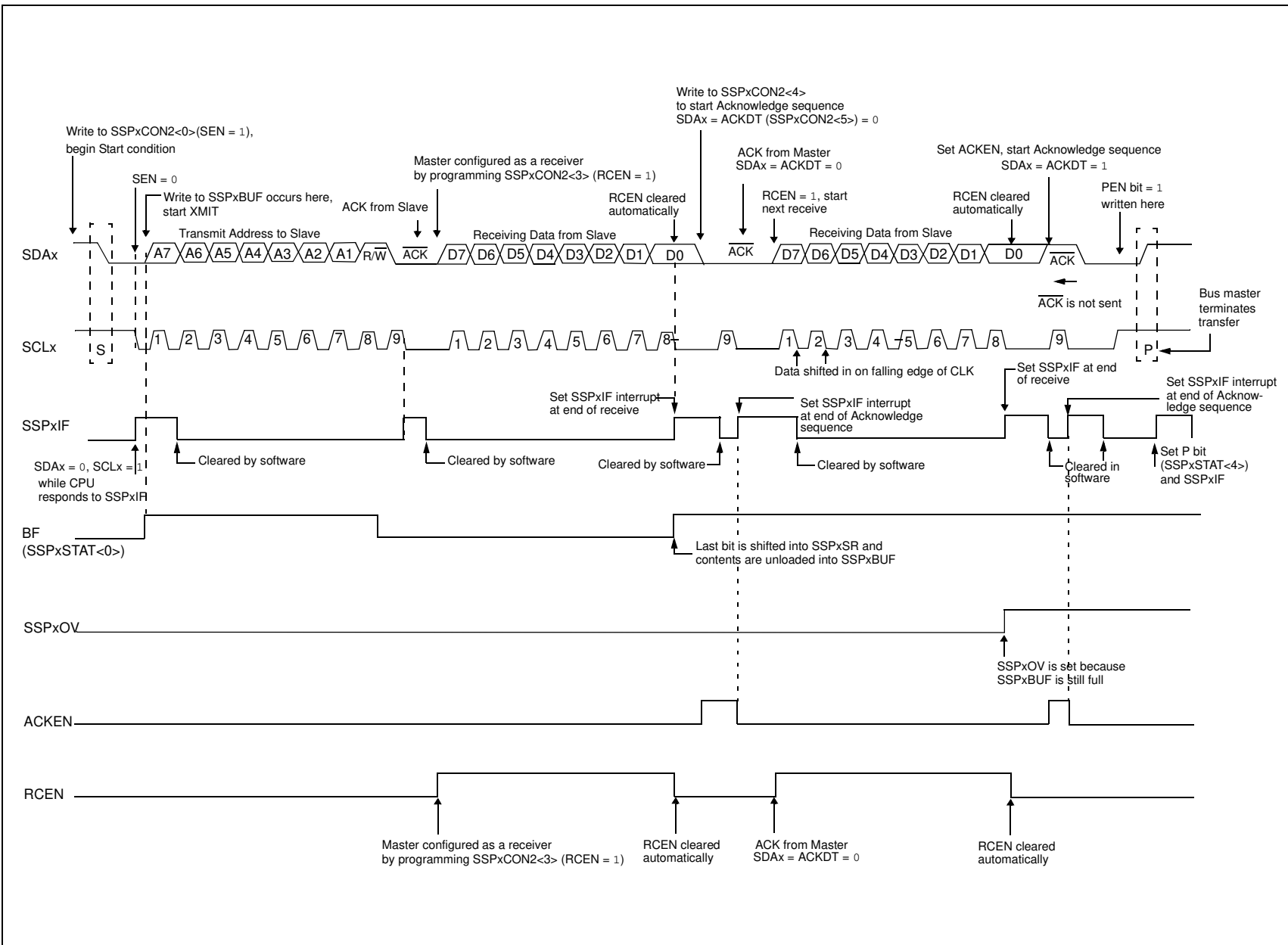
FIGURE 15-29: I 2 C™ MASTER MODE WAVEFORM (RECEPTION, 7-BIT ADDRESS)
