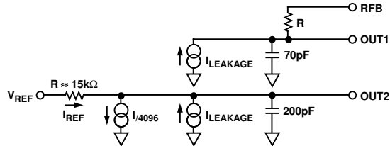
Figure 2. DAC Equivalent Circuit All Digital Inputs LOW
