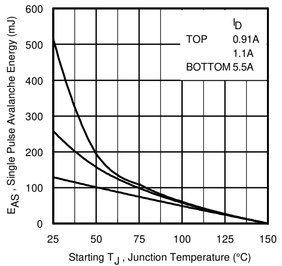
Fig 13a. Maximum Avalanche Energy vs. Drain Current
