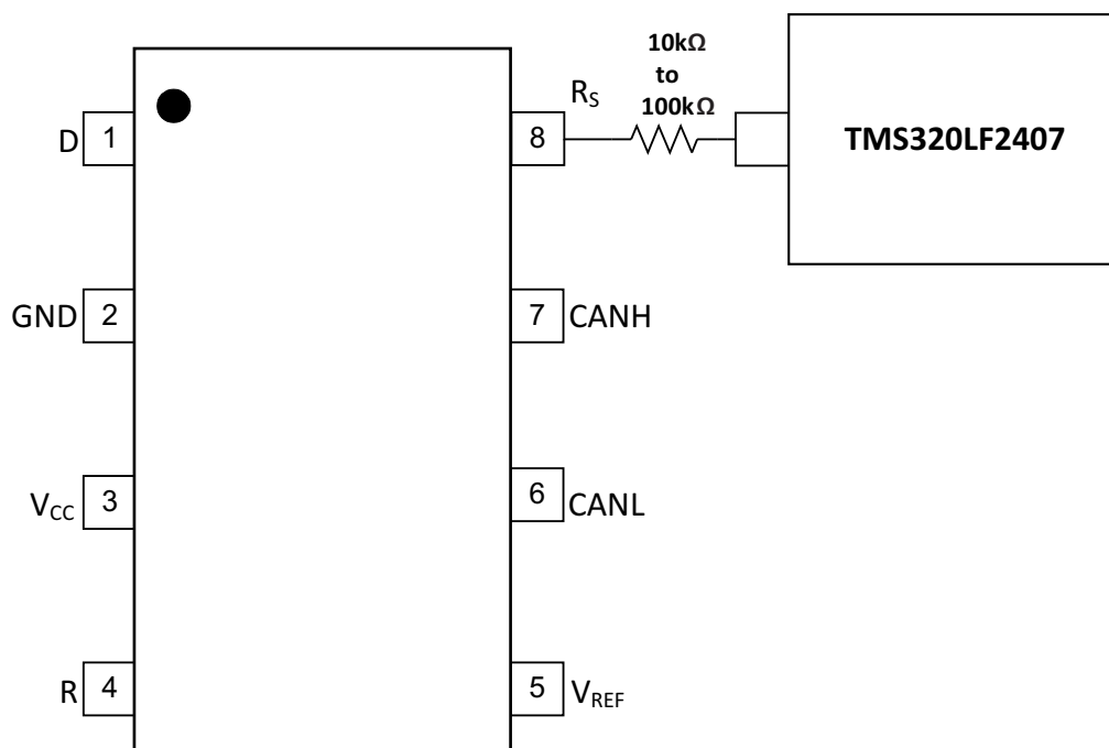
Figure 24. Slope Control
