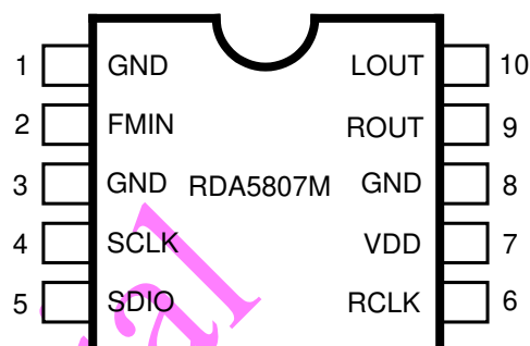
Figure1-1. RDA5807M Top View
