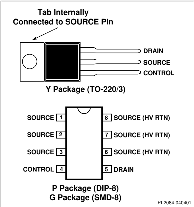
Figure 3. Pin Configuration.
