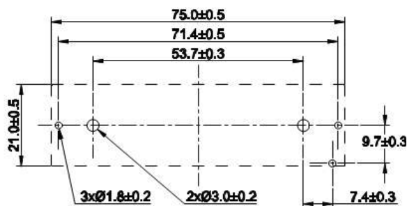
PCB/MOUNTING LAYOUT
