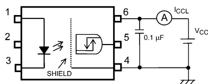
Fig. 12.1.3 ICCL Test Circuit
