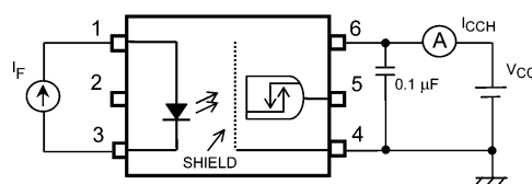
Fig. 12.1.4 ICCCH Test Circuit
