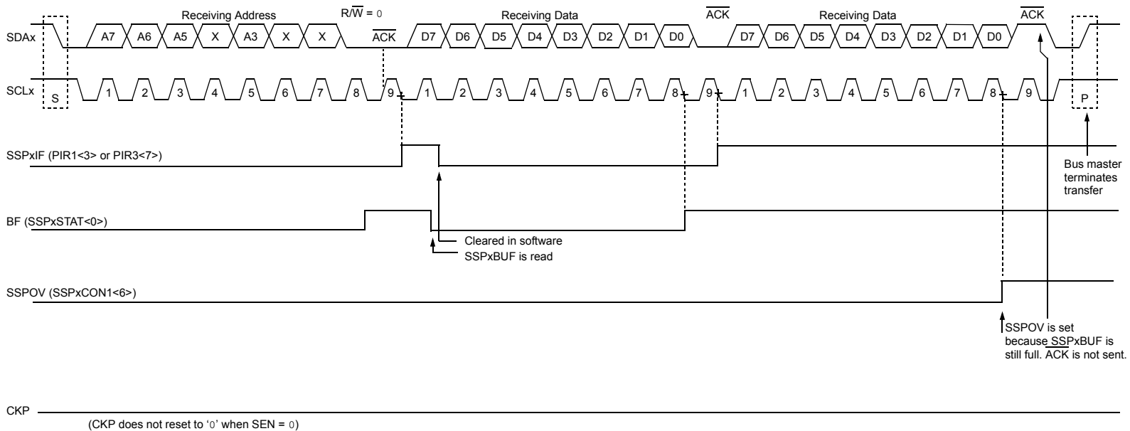
FIGURE 20-9: I 2 C™ SLAVE MODE TIMING WITH SEN = 0 AND ADMSK<5:1> = 01011 (RECEPTION, 7-BIT ADDRESS)
