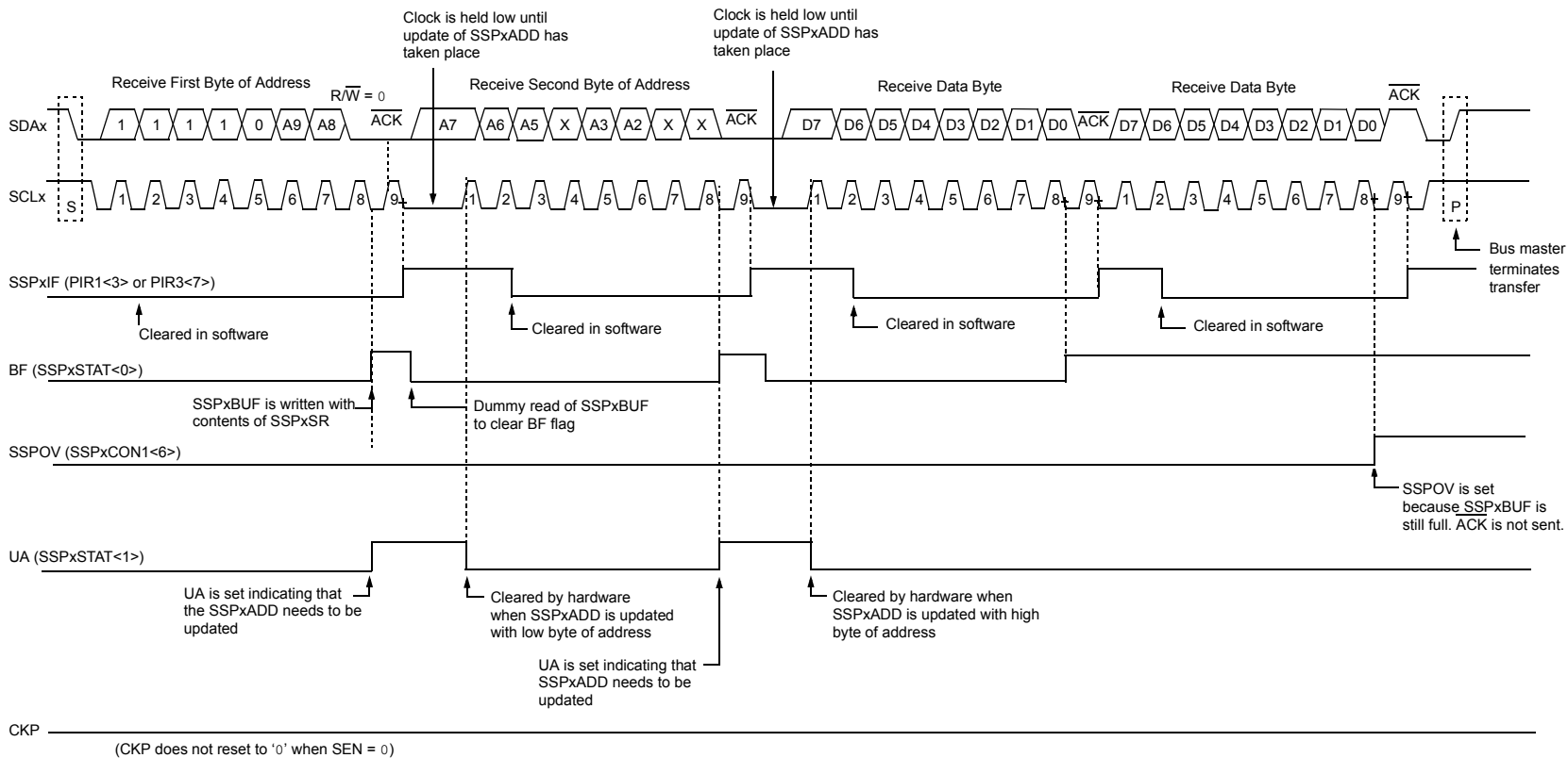
FIGURE 20-12: I 2 C™ SLAVE MODE TIMING WITH SEN = 0 AND ADMSK<5:1> = 01001 (RECEPTION, 10-BIT ADDRESS)
