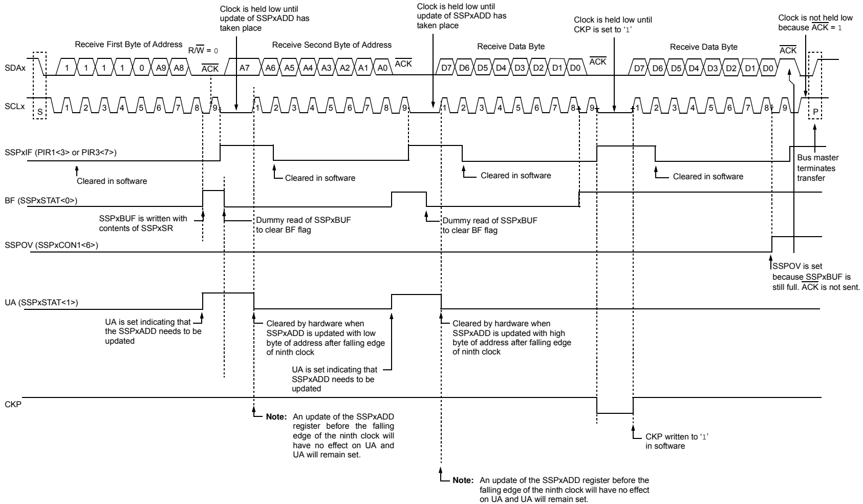
FIGURE 20-16: I 2 C™ SLAVE MODE TIMING WITH SEN = 1 (RECEPTION, 10-BIT ADDRESS)
