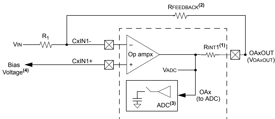
FIGURE 25-5: OP AMP CONFIGURATION A
