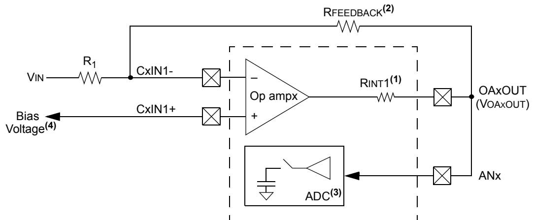
FIGURE 25-6: OP AMP CONFIGURATION B
