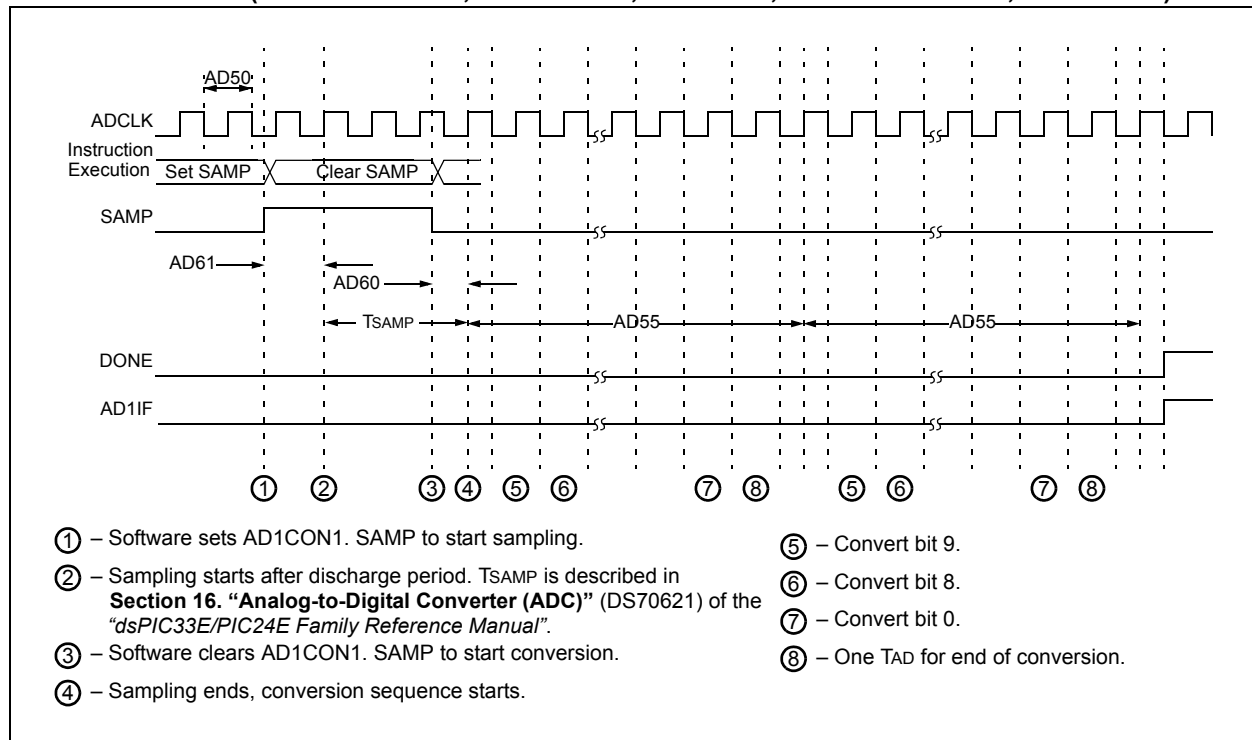
FIGURE 30-37: ADC CONVERSION (10-BIT MODE) TIMING CHARACTERISTICS (CHPS<1:0> = 01, SIMSAM = 0, ASAM = 0, SSRG<2:0> = 000, SSRG = 0)
