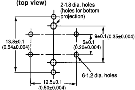
PCB mounting (top view)
