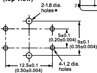
PCB mounting (top view)
