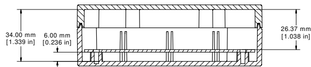
SECTION B-B
