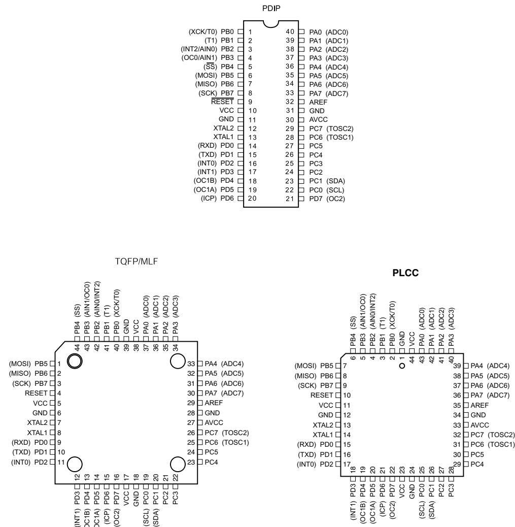
Figure 1. Pinout ATmega8535
