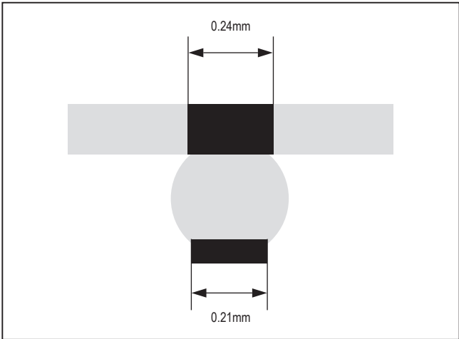
Figure 21. MAX98357A/MAX98357B WLP Ball Dimensions
