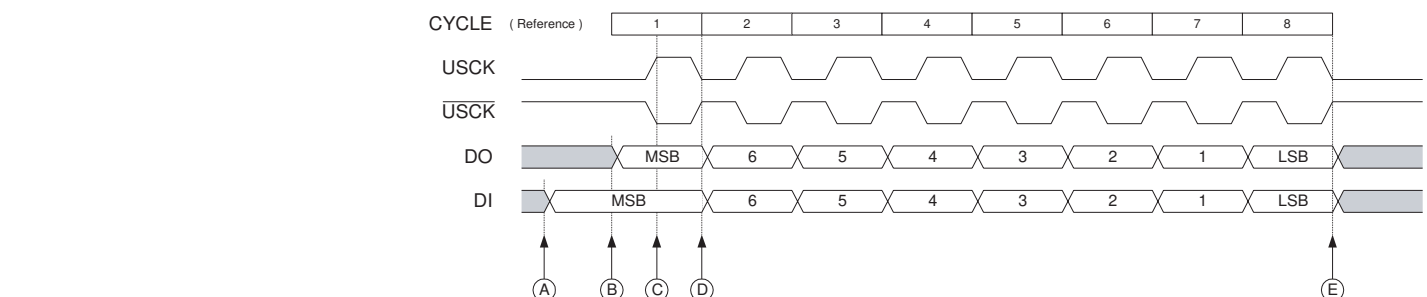
Figure 62. Three-wire Mode, Timing Diagram
