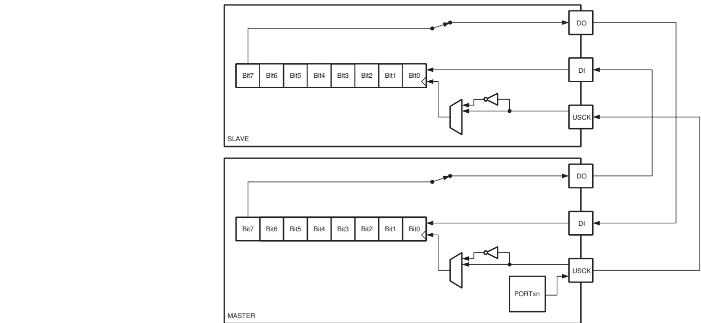
Figure 61. Three-wire Mode Operation, Simplified Diagram
