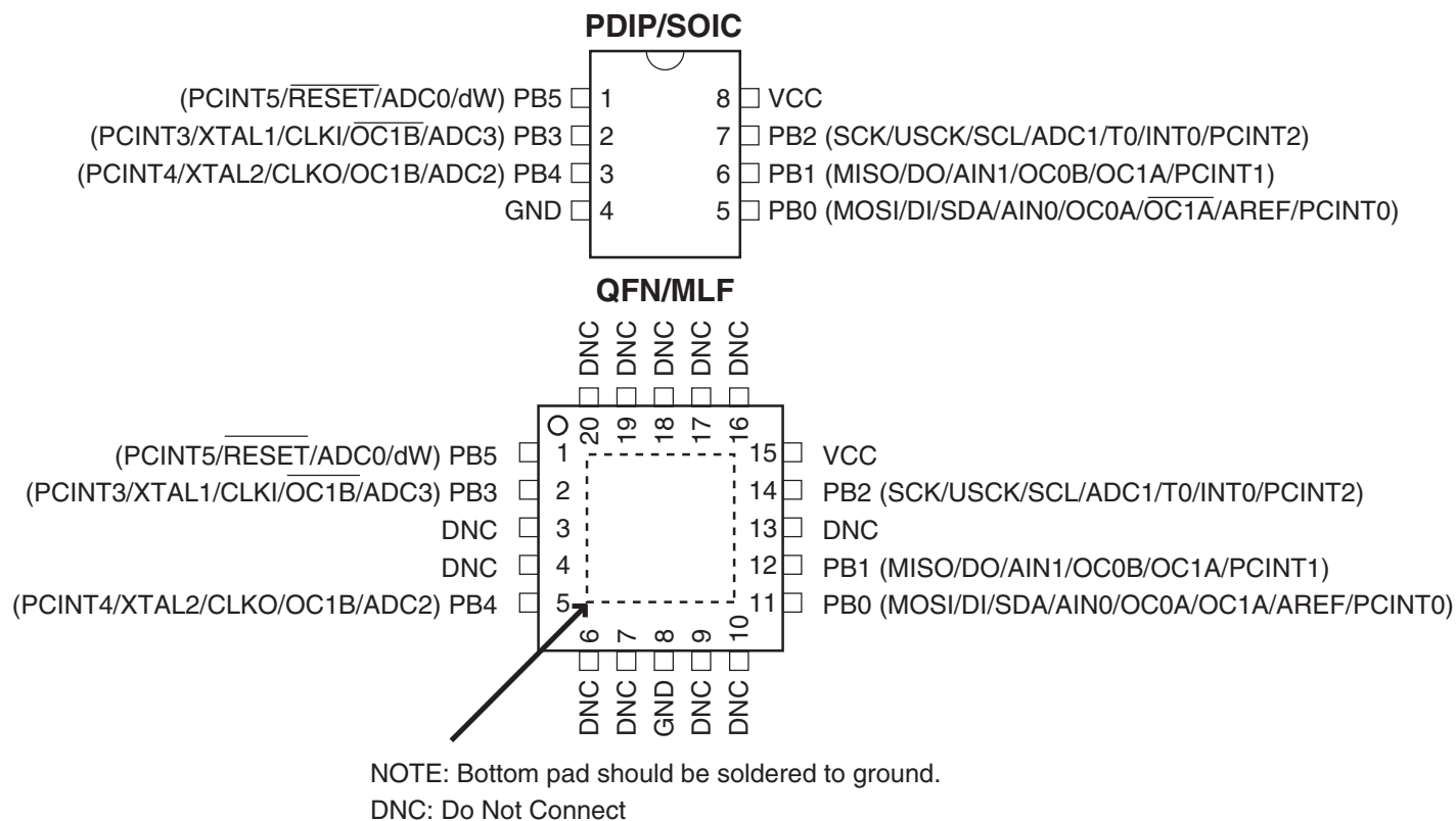
Figure 1-1. Pinout ATtiny25/45/85
